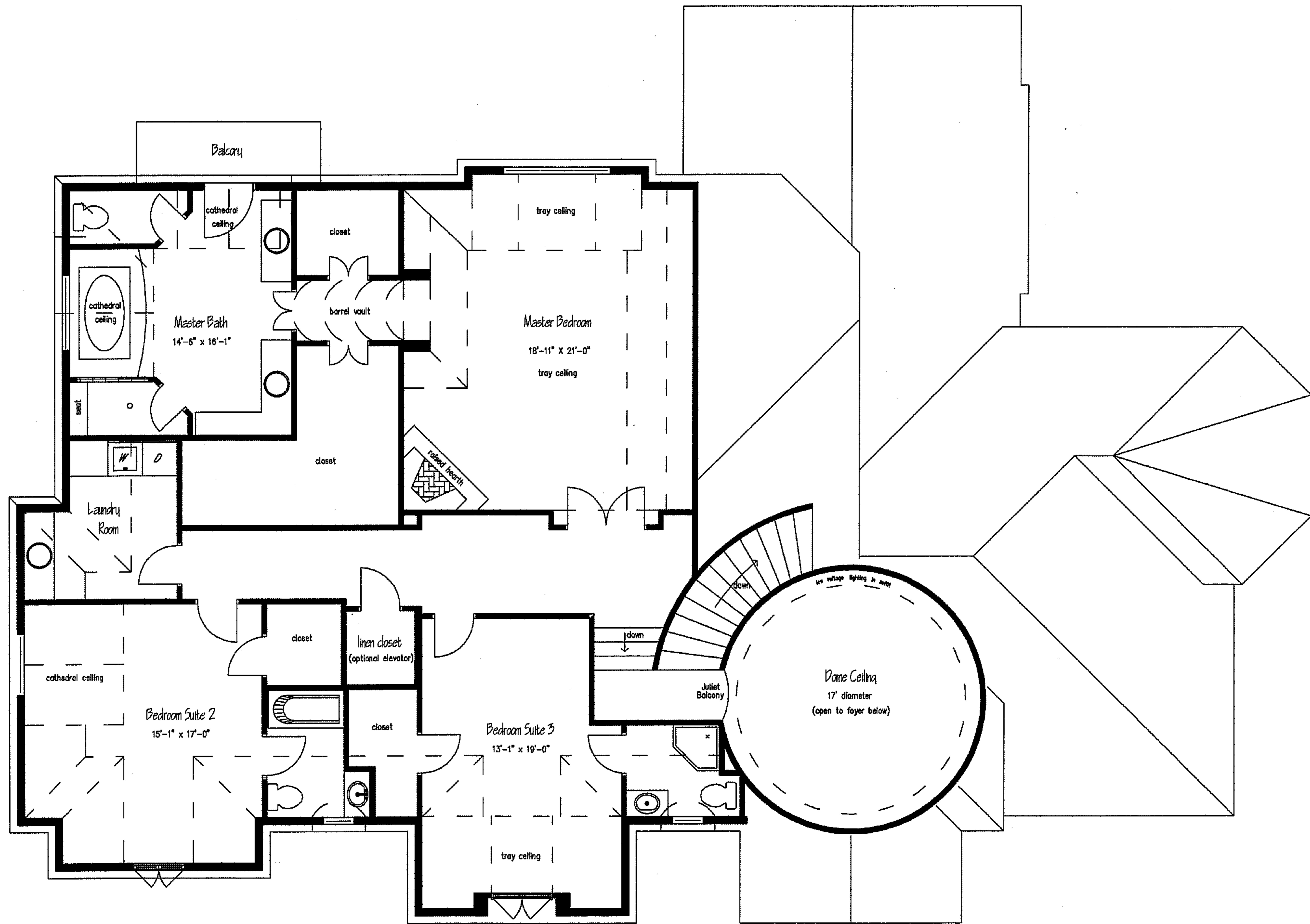
UPPER FLOOR PLAN, 1043 METEOR PLACE
