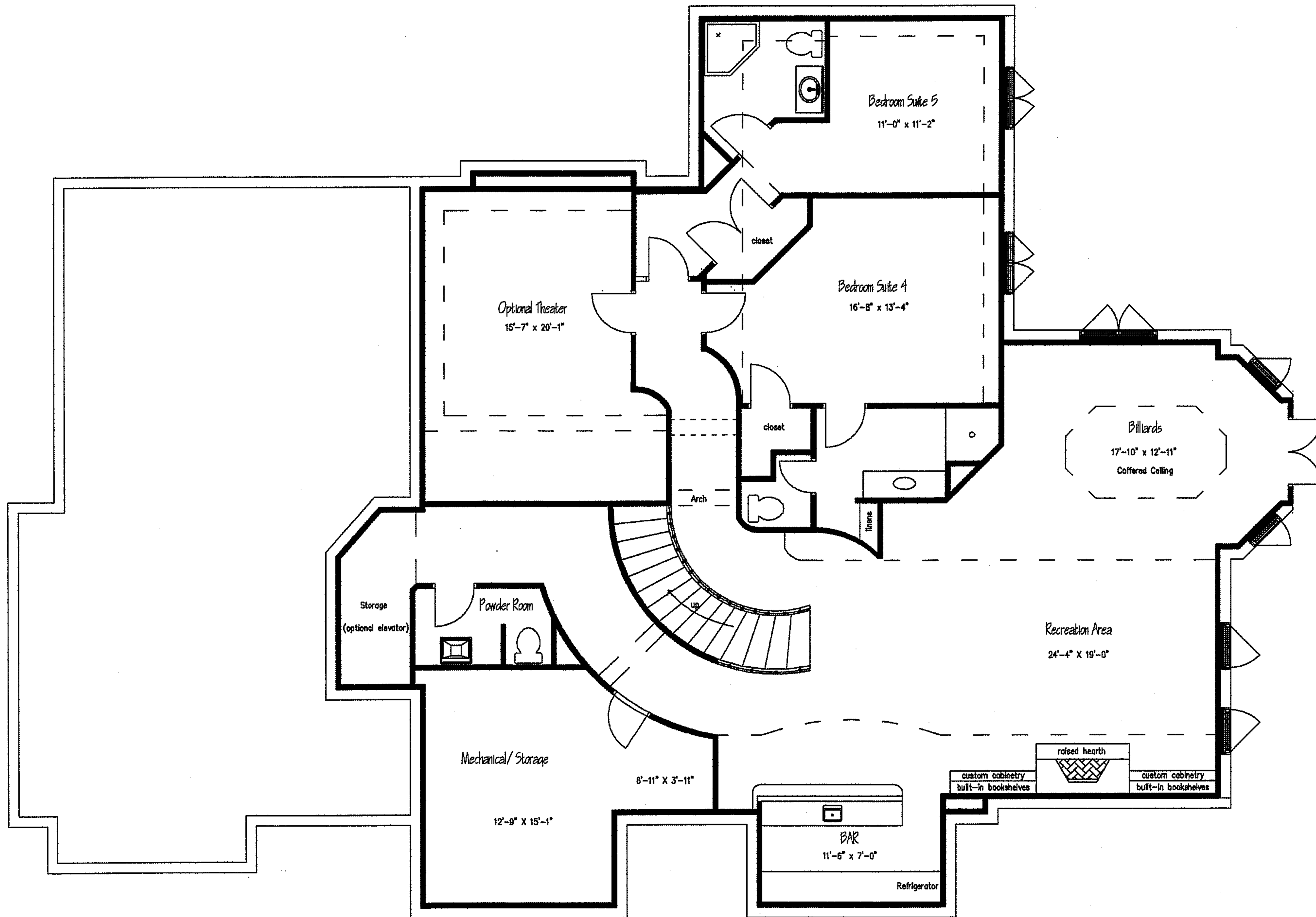
LOWER FLOOR PLAN, 1043 METEOR PLACE
